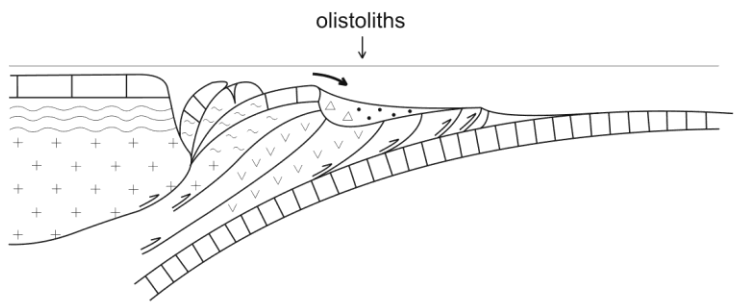
Fig. 3 Conceptual geodynamic and sedimentation model for the Middle Jurassic evolution of the region studied.
